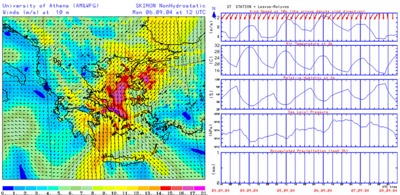
Fig. 3 72nd-hSKIRONforecast of the wind field over Greece on September 6, 2004 at 12UTC and meteograms for the whole 120-h forecasting period for Lesvos Island
