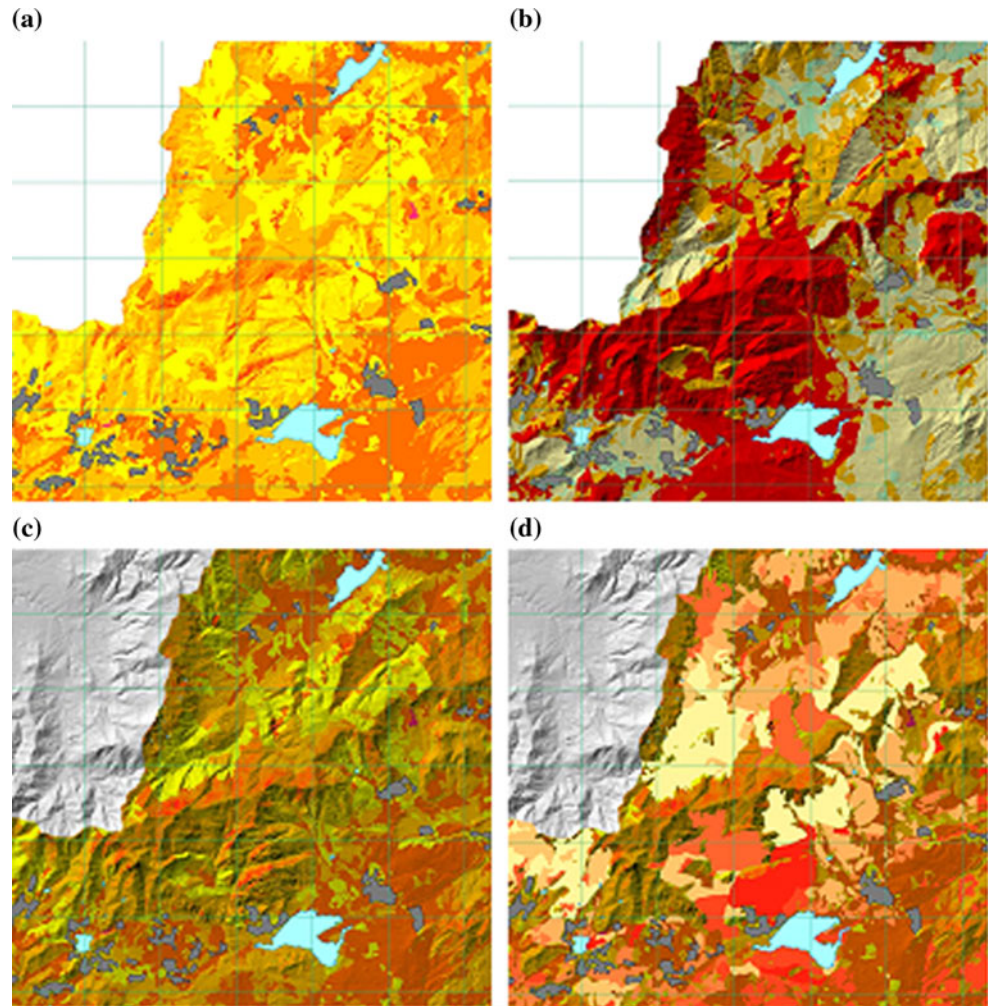
Fig. 5 Maps of (a) linear fire intensity; (b) potential crown fire; (c) rate of fire spread; and (d) potential fire loss index in resolution of 20 m
