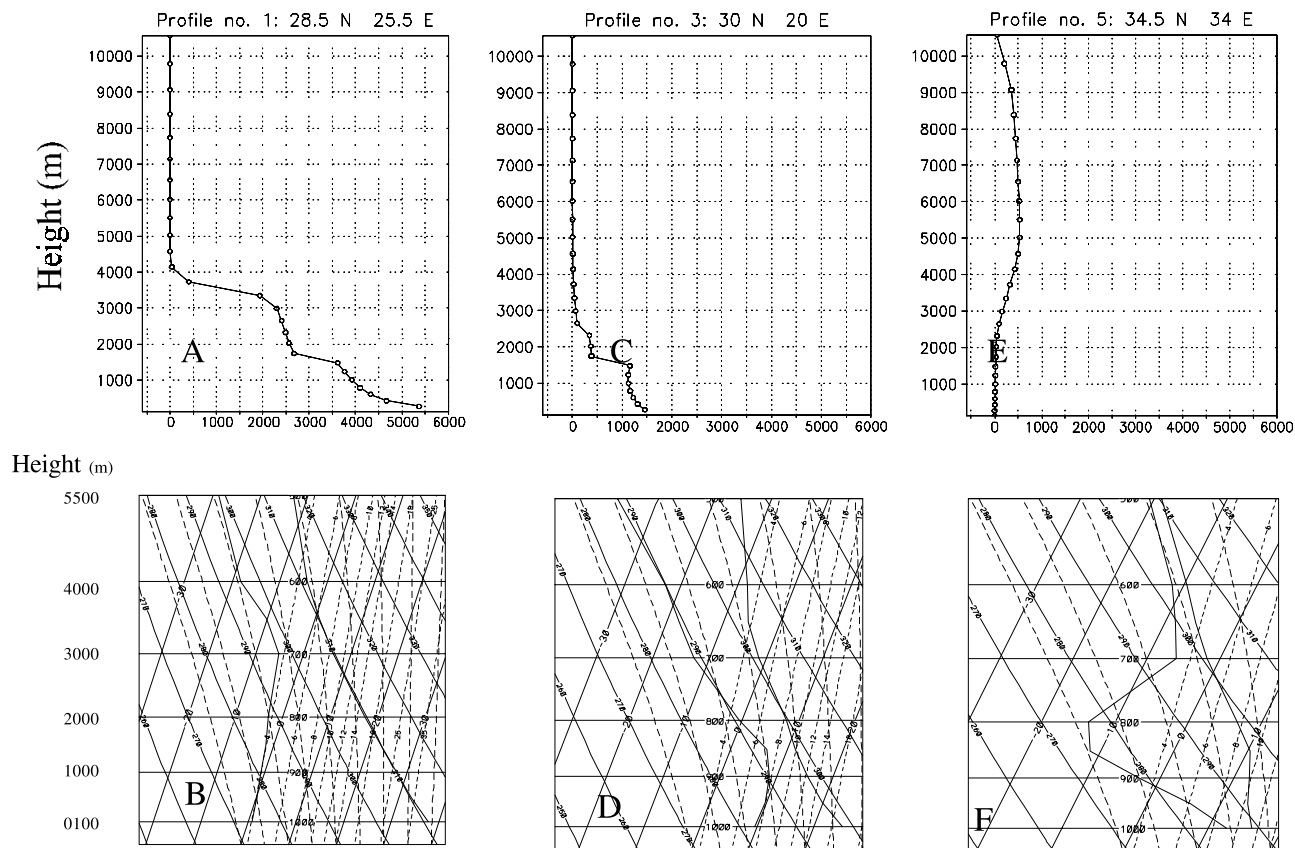
Figure 7. Vertical dust concentrations as well as temperature and dew point temperature profiles simulated for three locations indicated in Figure 5 at 1200 UTC 15 March, 1998. (a, c, and e) dust concentrations at locations 1, 3, and 5, respectively. (b, d, and f) temperature and dew point temperature profiles at the 1, 3, and 5 locations.
